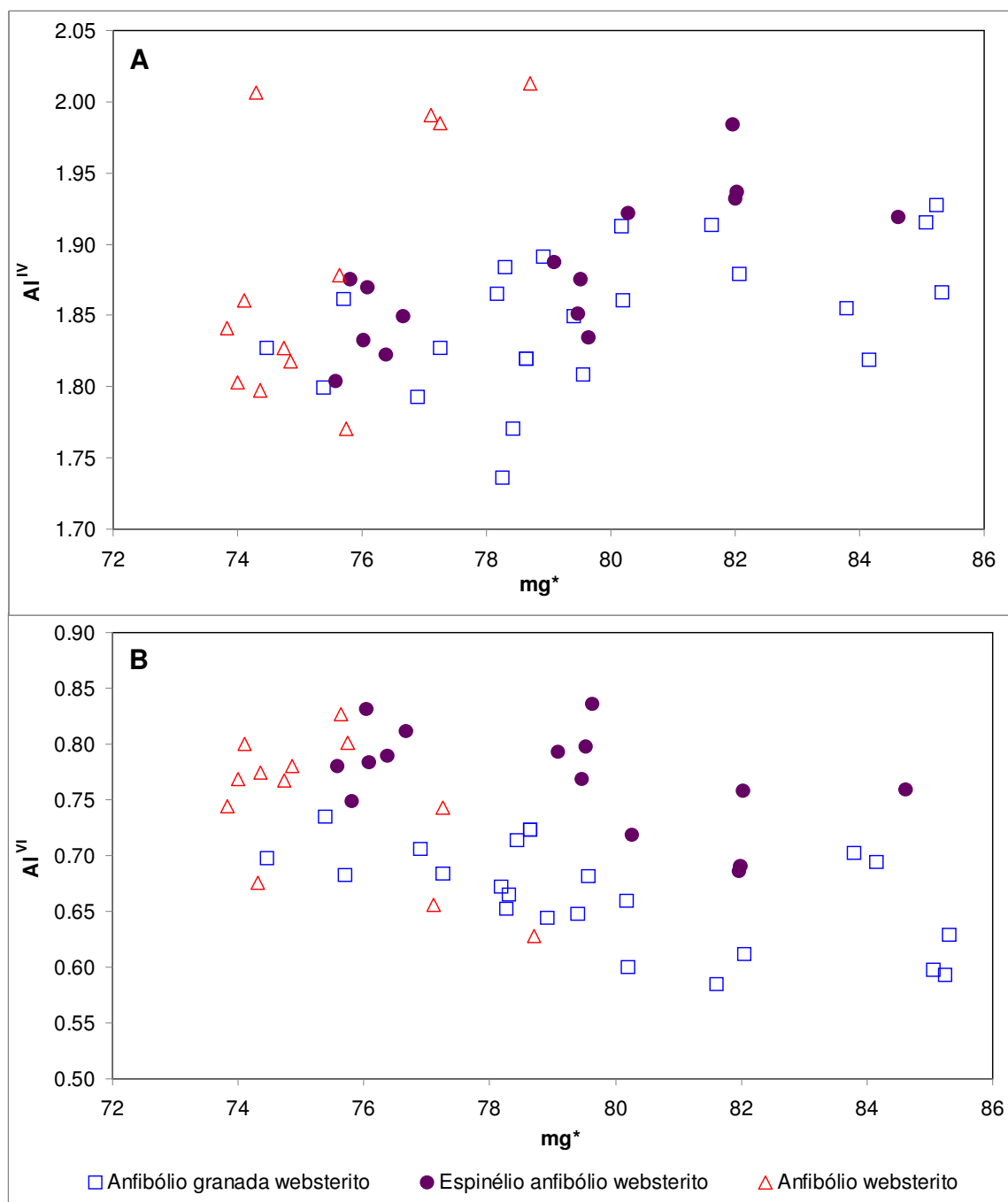
Figura 5.7.4. Diagramas mg\# versus Al^{IV} (A) e mg\# versus Al^{VI} (B).
